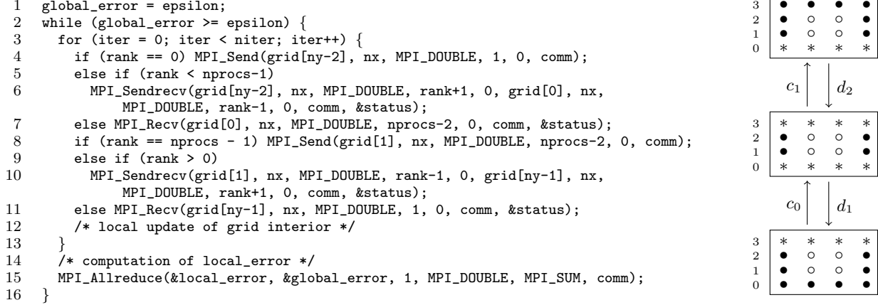
Figure 1: Jacobi iteration on a two-dimensional grid: \bullet = boundary cell, \circ = interior cell, * = ghost cell
